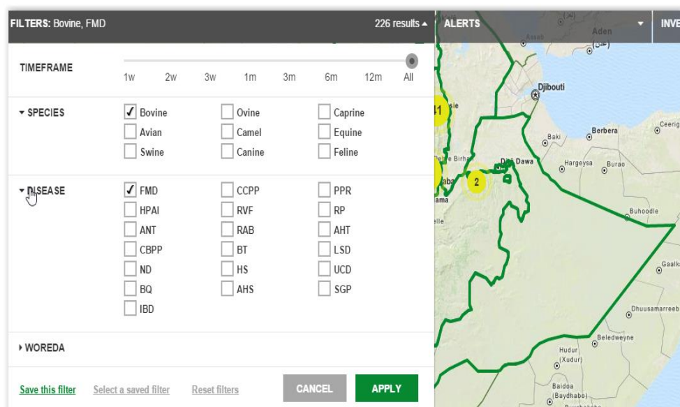
Figure 14: Applying Filters
