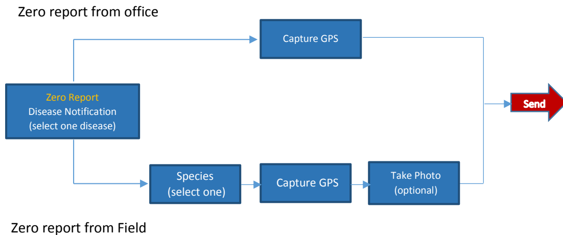
Figure 1: Zero Reporting
